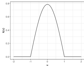
Cosine kerel
