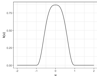
Tricube kerel
